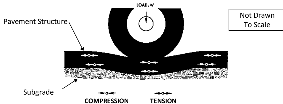
Figure 3-2 Pavement Deflection Results In Tensile and Compressive Stresses In Pavement Structure
