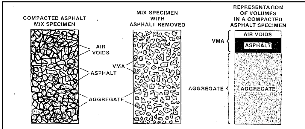
Figure 4-2 Illustration of VMA in a Compacted Mix Specimen
