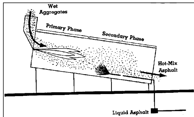
Figure 6-18 Zones in Drum Mixer
