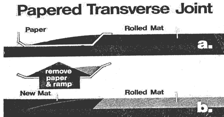
Figure 9-20 Paper Joint
