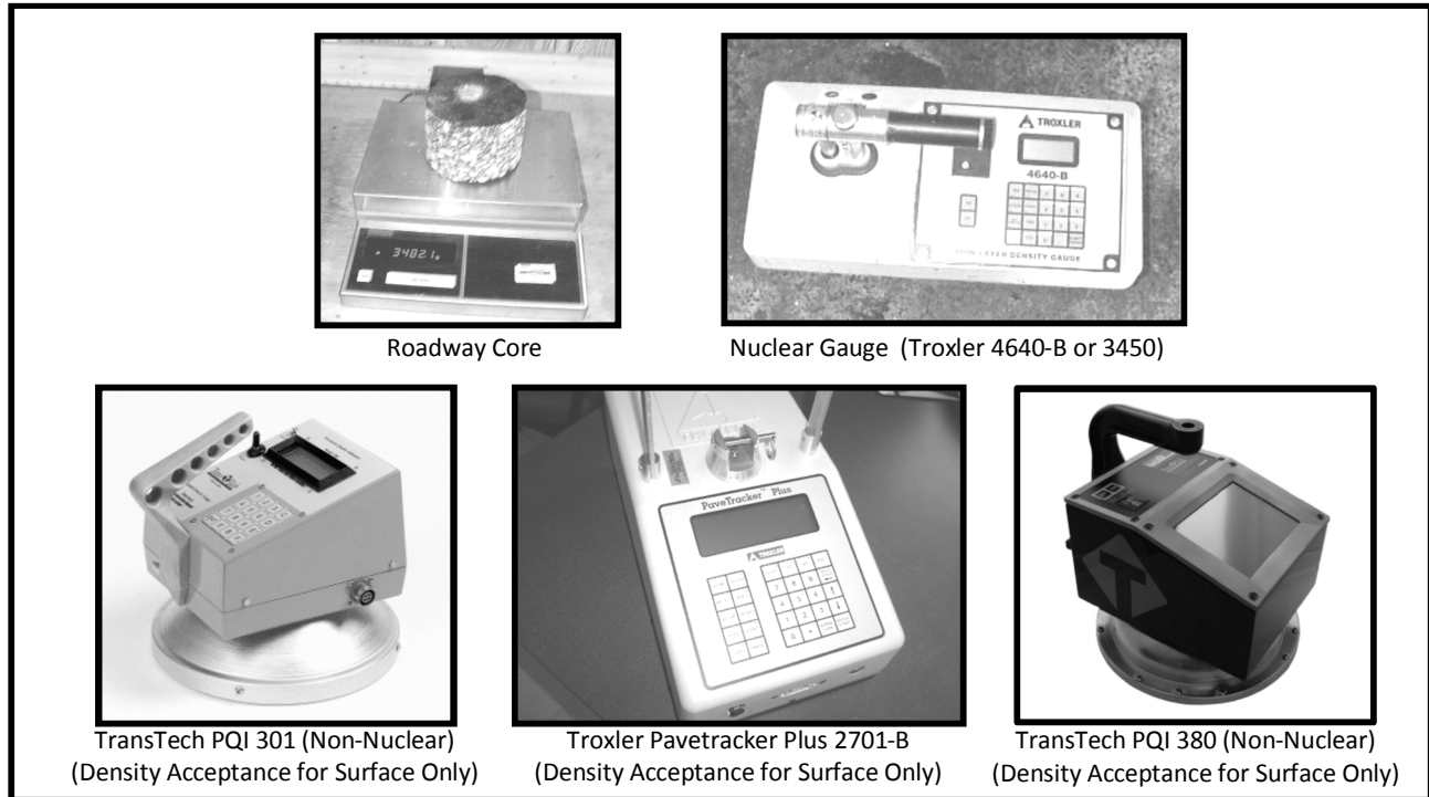
Figure 10-1 Density Test Methods
