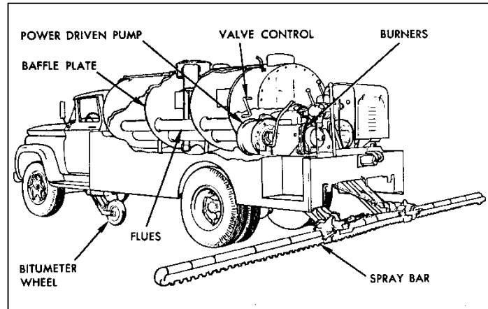
Figure 9-1 Asphalt Distributor
