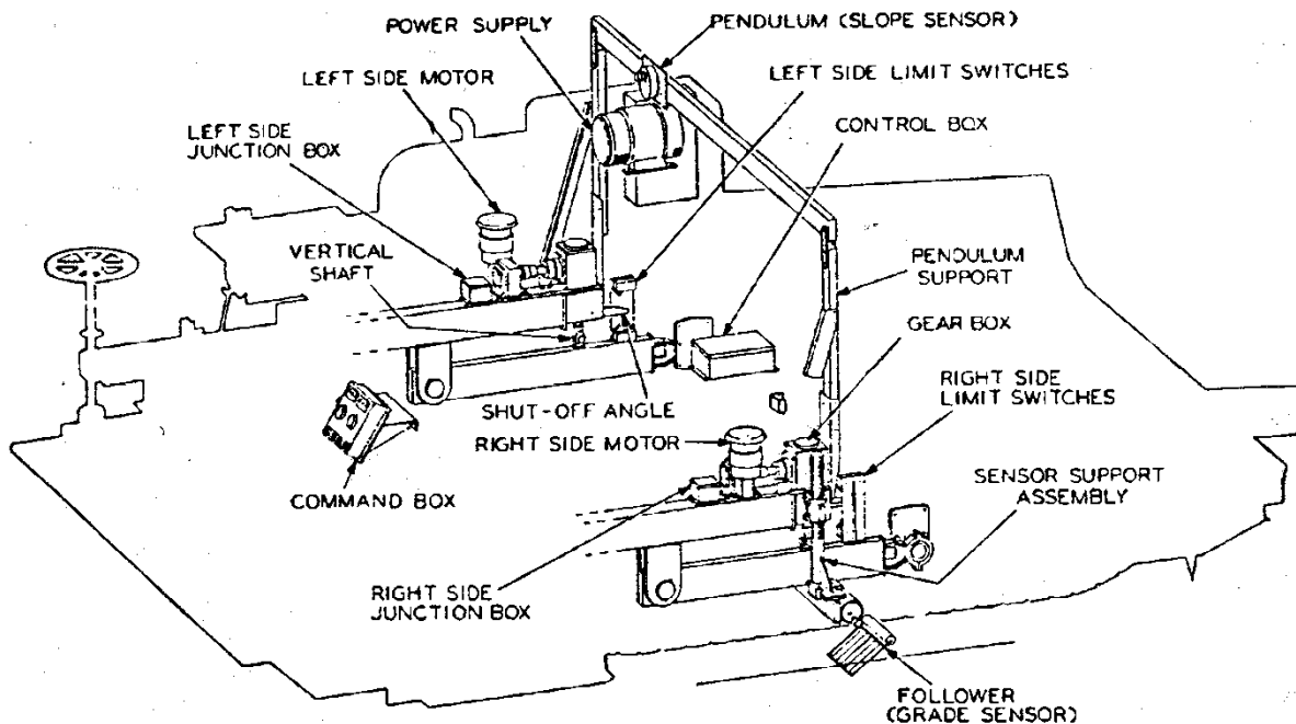
Figure 9-7 Components of an Automatic Screed Device
