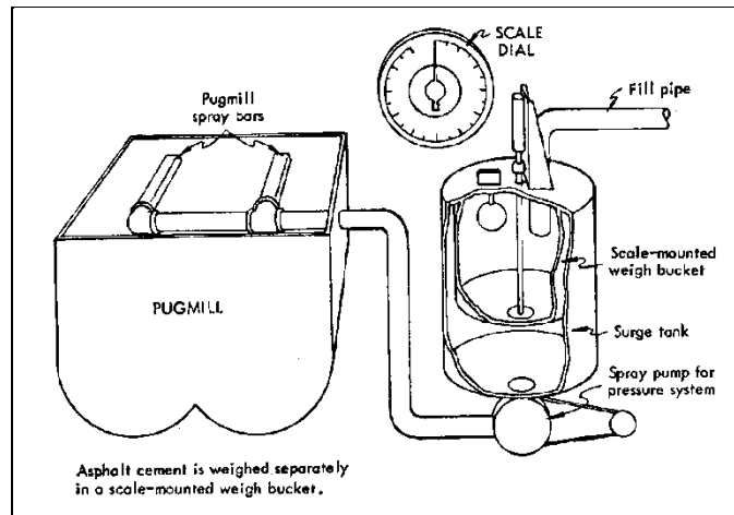
Figure 6-16 Typical Asphalt Binder Measuring and Delivery System
