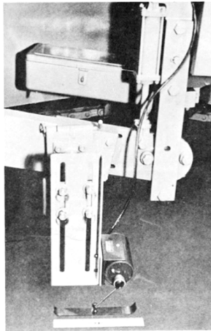
Figure 9-9 Long Mobile Grade Reference System (Sonic Type with 4 Referencing Sensors)
