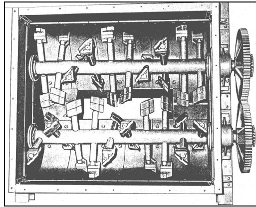
Figure 6-10 Pugmill Mixer for a Batch Plant
