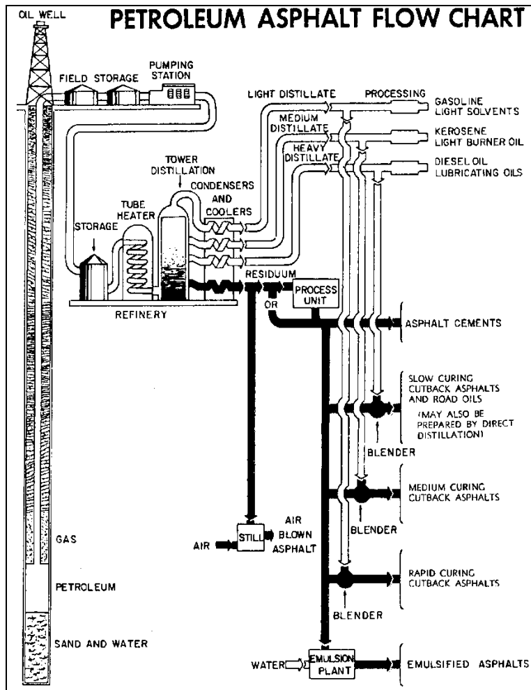
Figure 2-1 Typical Refining Process
