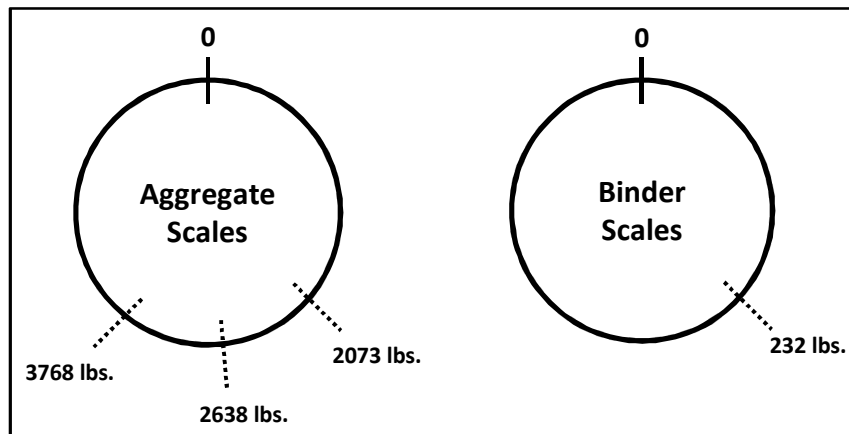
Figure 6-15 Asphalt Plant Scale Settings
