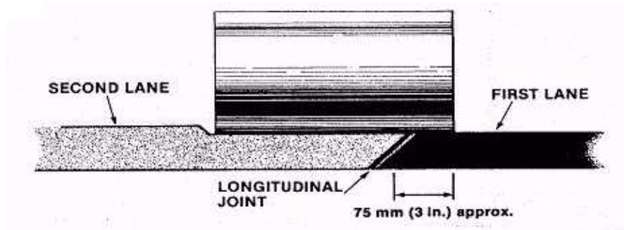
Figure 9-25 Joint Rolling Procedure
