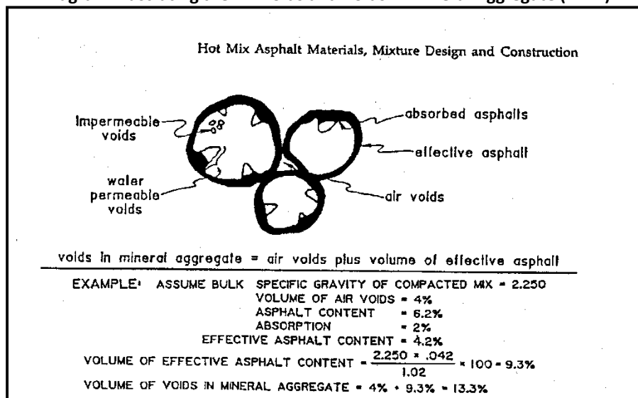
Figure 4-3 Diagram Illustrating the Air Voids and Voids in Mineral Aggregate (VMA)
